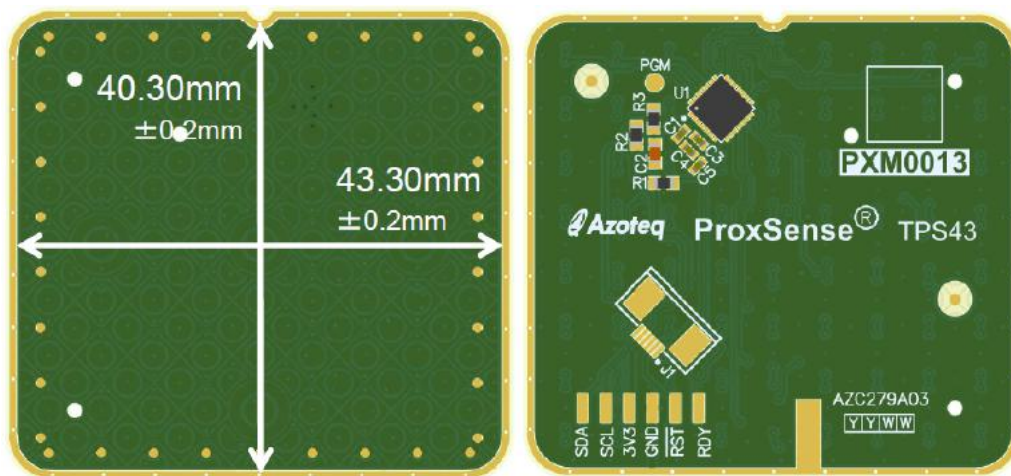
Figure 2.1: TPS43 – Module representation for metal dome overlay
