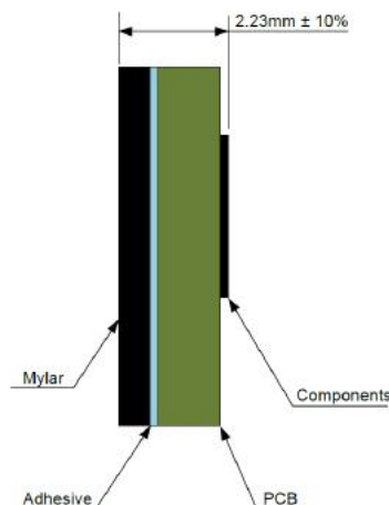
Figure 1.2: Stack-Up (B) - Thickness: PCB + 3M double sided adhesive + Mylar overlay
