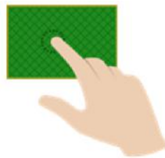
Figure 4.2: Tap gesture
