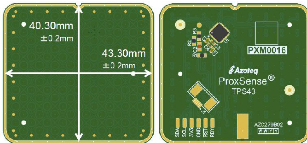
Figure 2.2: TPS43 – Module representation for mylar overlay
