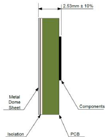
Figure 1.3: Stack-Up (C) - Thickness: PCB + isolation + metal dome sheet
